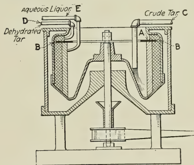
FIG. 74.—Centrifugal Tar Dehydrator.
